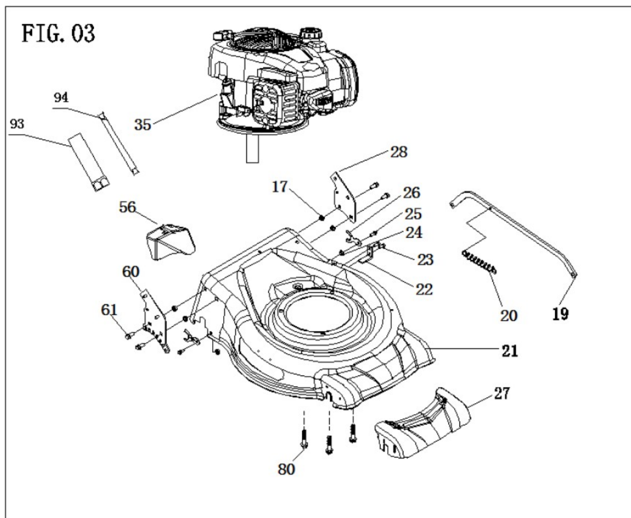
Fig.03 Governor Group
