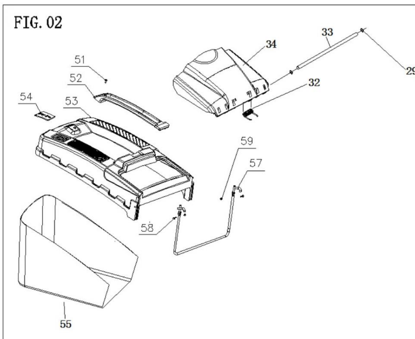
Fig. 02 Grass Catcher Group
