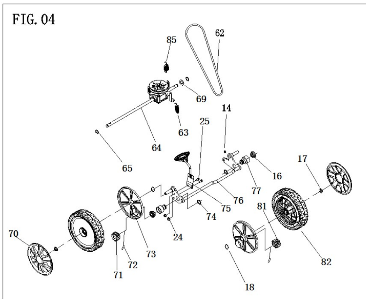
Fig. 04 Running Group
