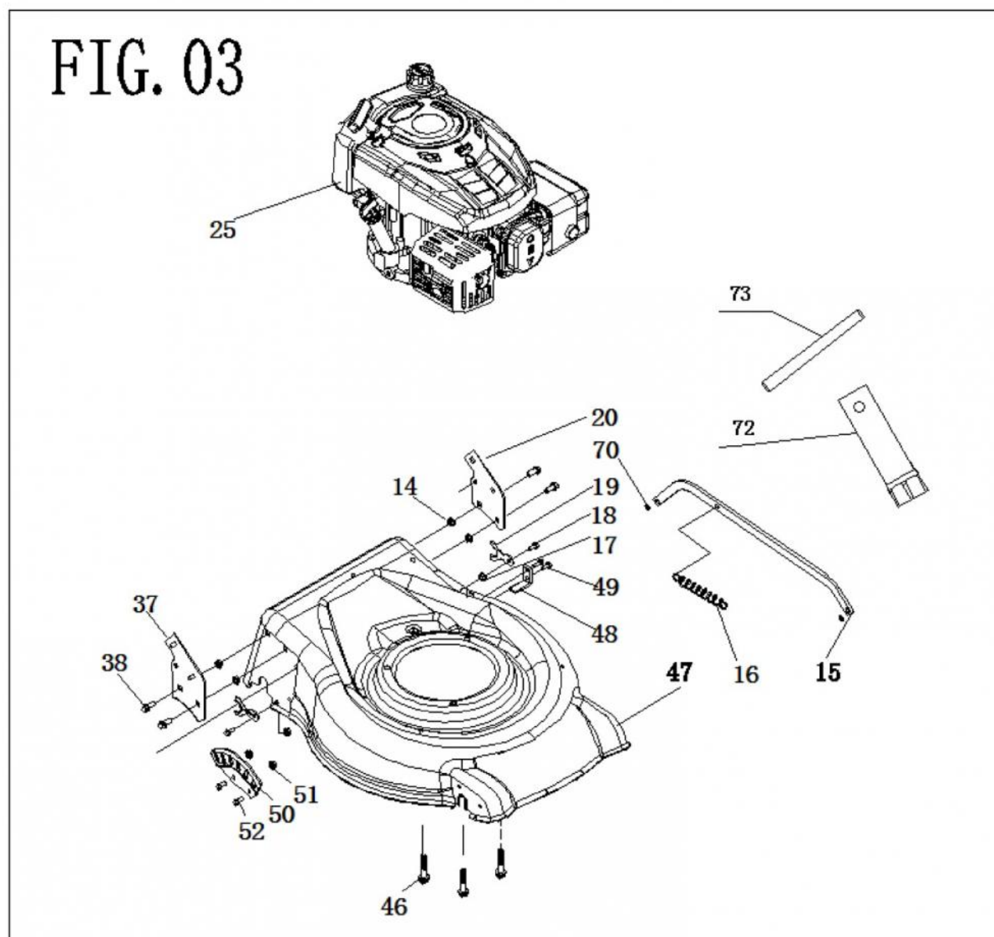
Fig.03 Governor Group
