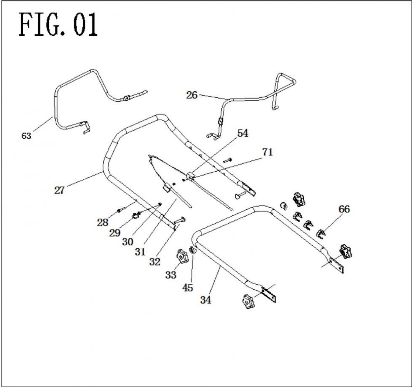
FIG.01 Operating Group
