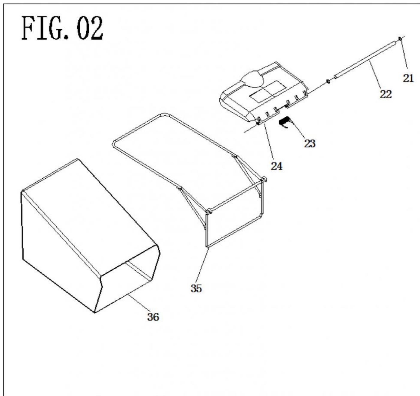
Fig. 02 Grass Catcher Group
