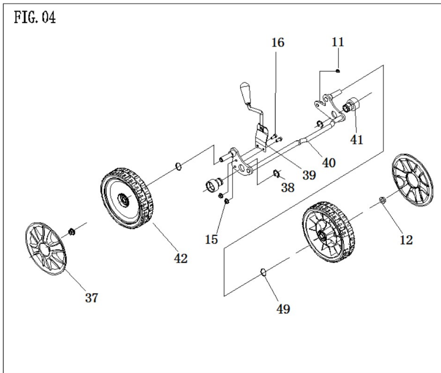
Fig. 04 Running Group
