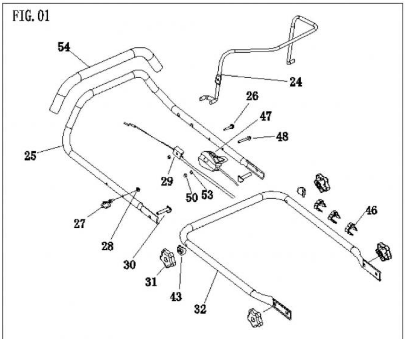
FIG.01 Operating Group
