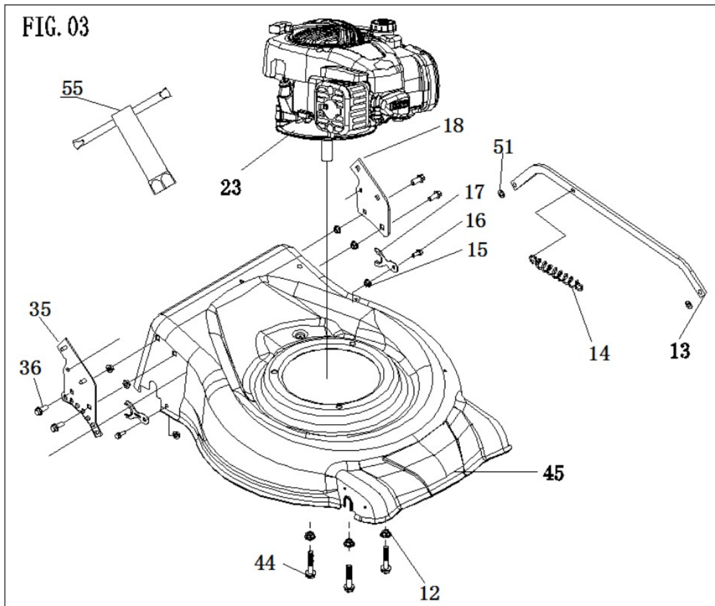
Fig.03 Governor Group
