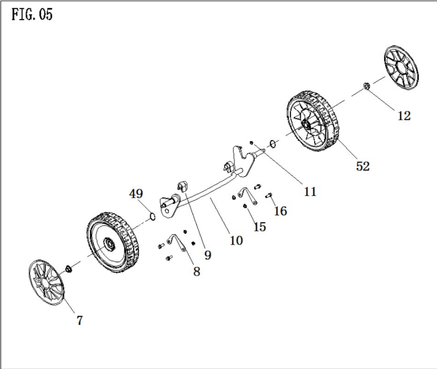
Fig. 05 Running Group
