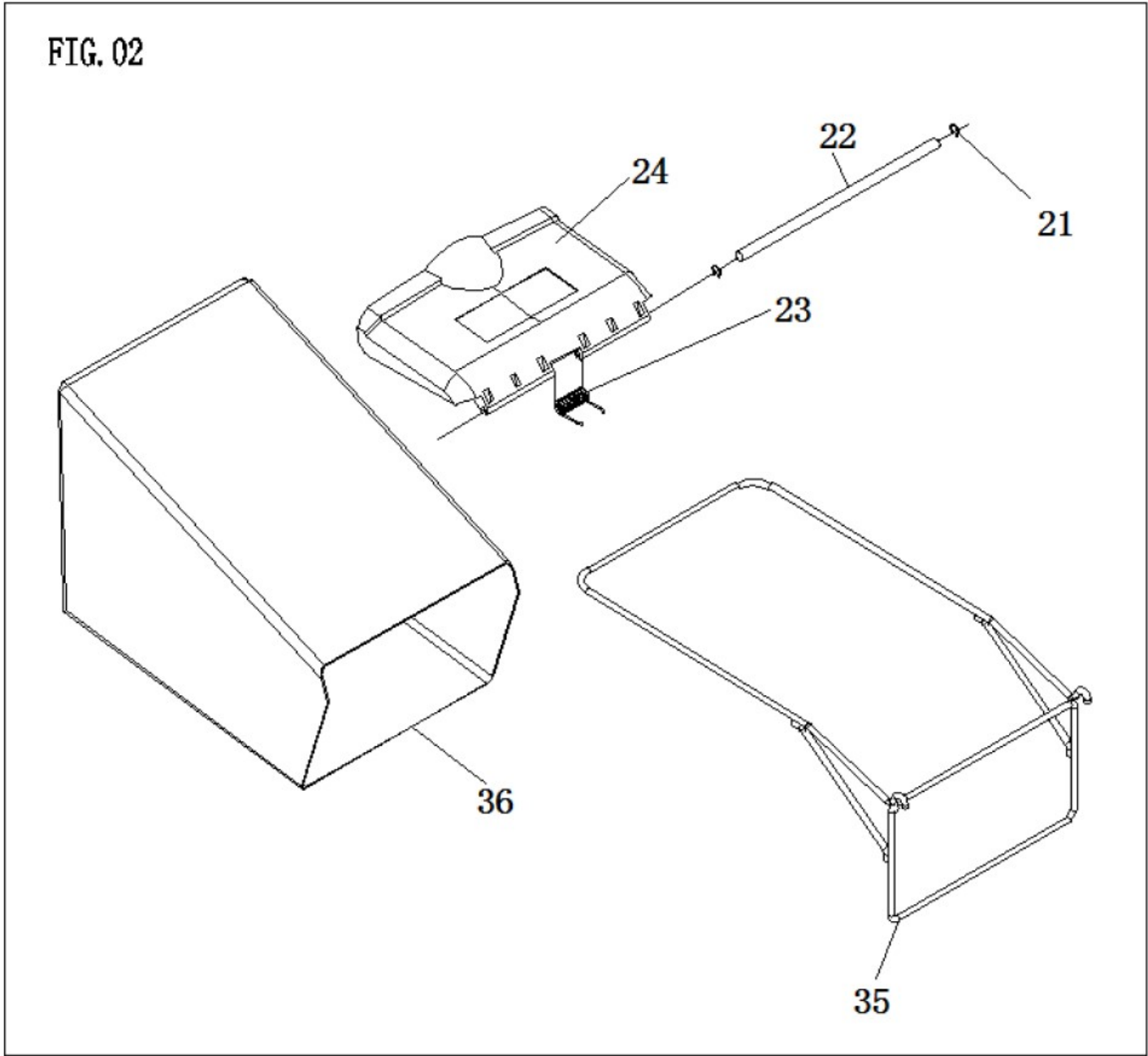
Fig. 02 Grass Catcher Group
