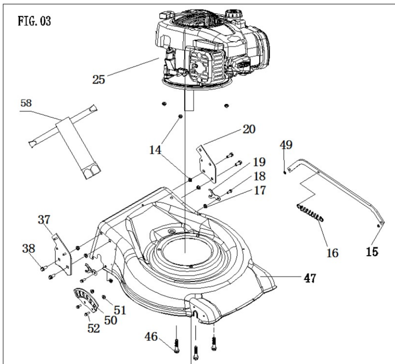
Fig.03 Governor Group
