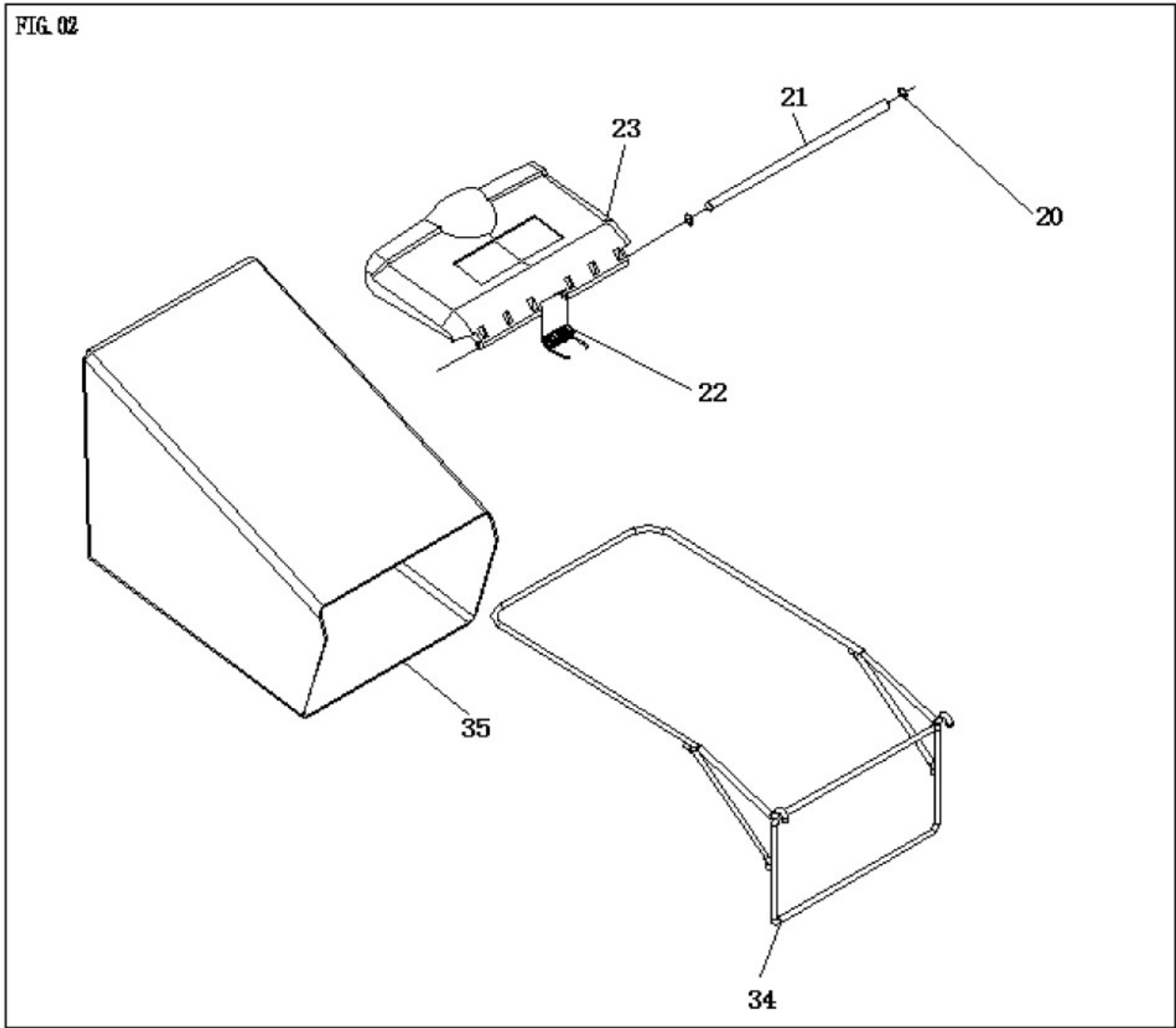
Fig. 02 Grass Catcher Group
