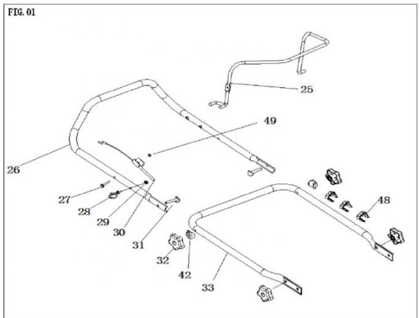
FIG.01 Operating Group
