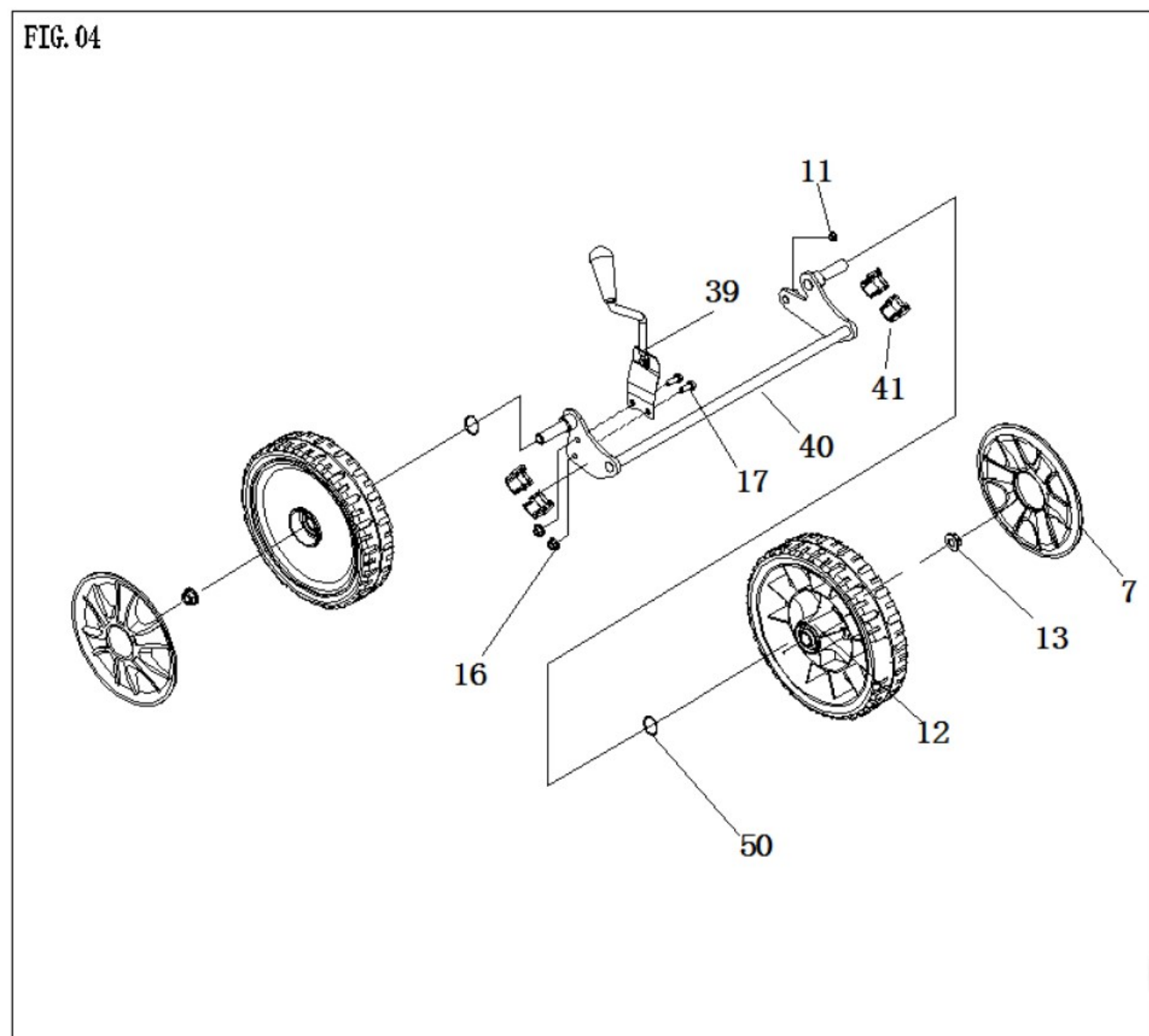
Fig. 04 Running Group
